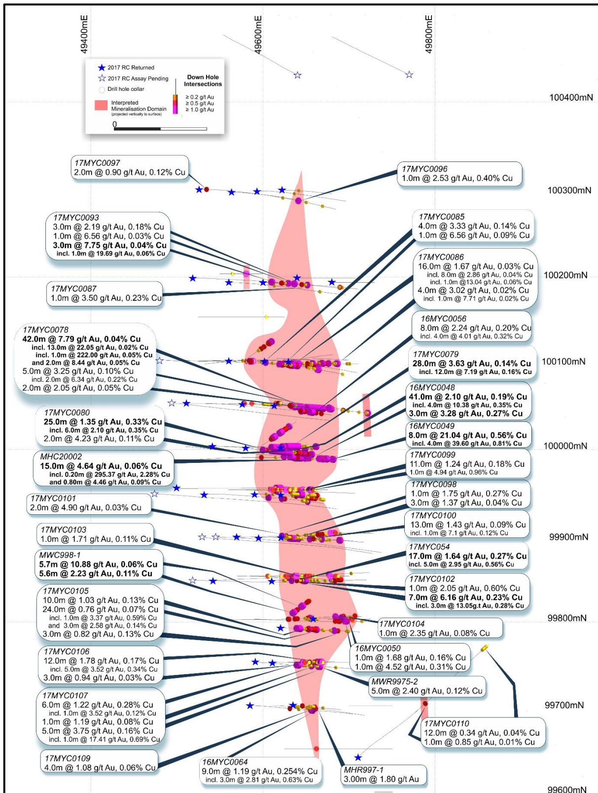
Figure 2: WACA Deposit plan view showing drill hole locations and generalised plan projection of approximate boundary encapsulating 1.0 g/t gold mineralisation. Note: Labelled 2017 Phase 1 RC drill hole intercepts in blue (100m NS and 200m EW Local Grid).
