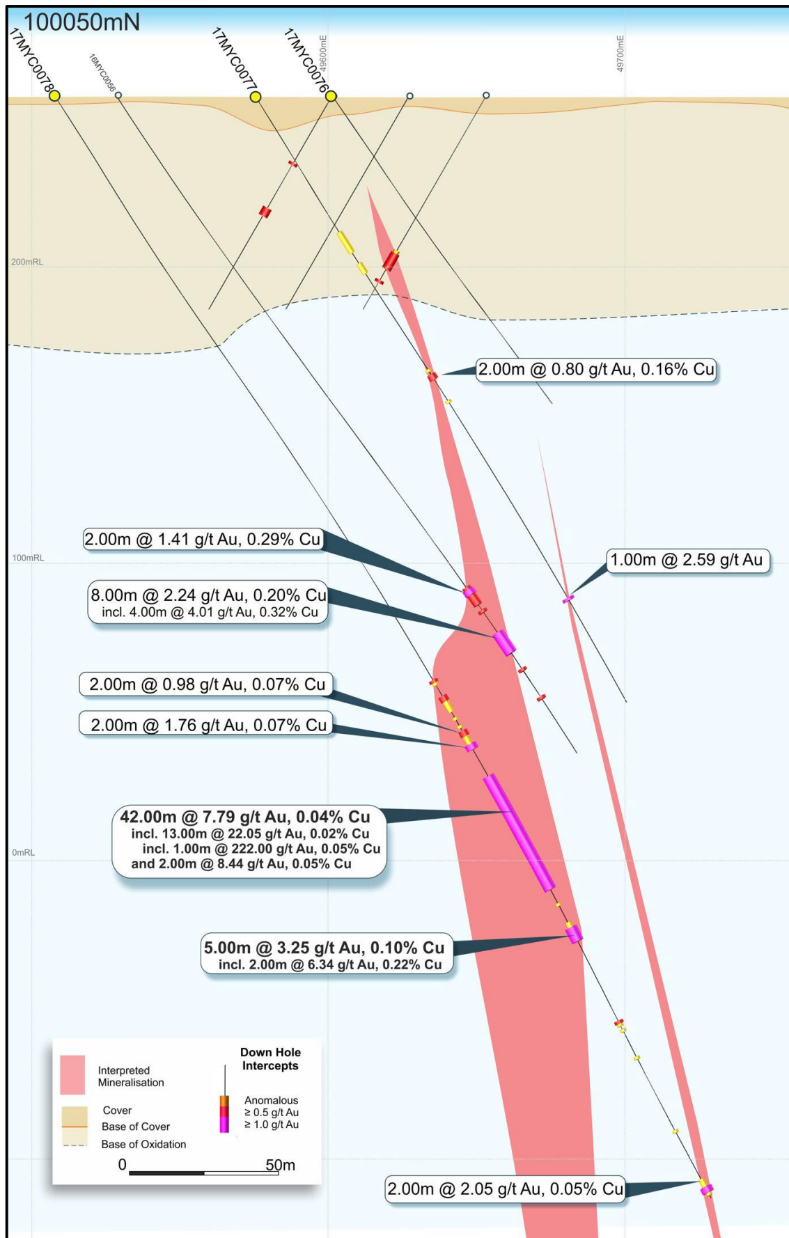
Figure 4: WACA Deposit 100,050 North interpreted (schematic) cross-section showing drill holes, including 2017 Phase 1 RC drill holes, with gold grade bars and interpreted gold-copper mineralisation domains (100m Local Grid – looking north).
