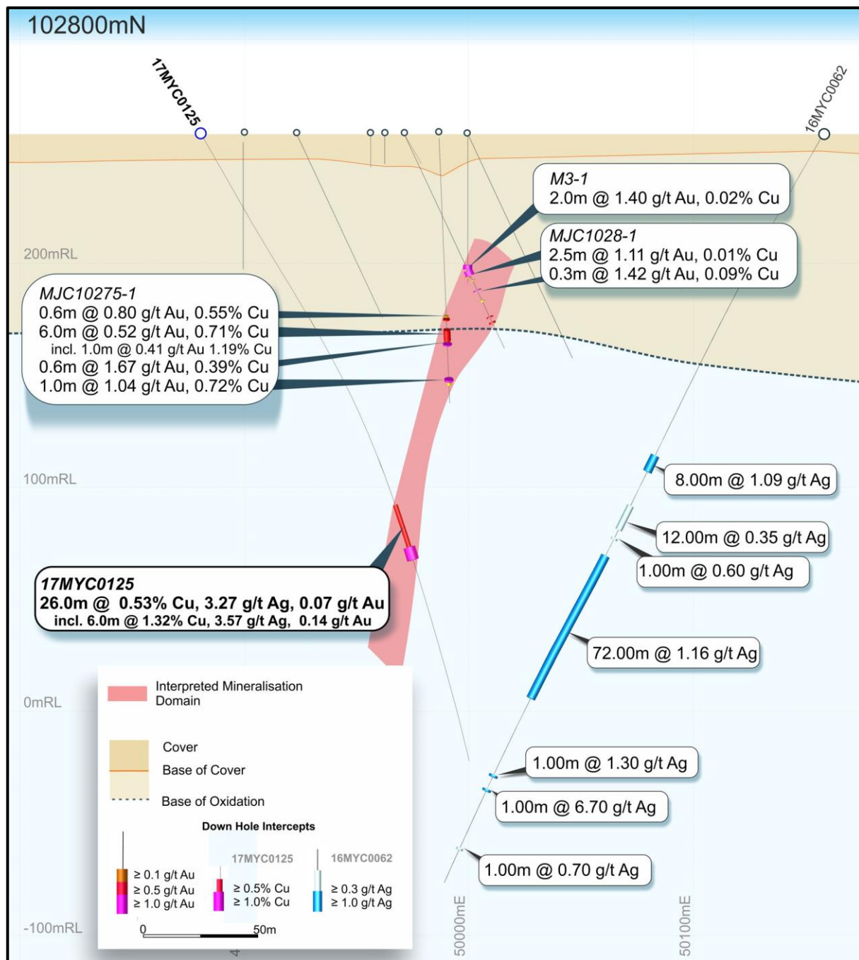
Figure 6: Jude's area 102,800 North interpreted (schematic) cross-section showing drill holes, including 2017 Phase 1 RC drill hole, with mineralisation grade bars and interpreted copper-silver-gold mineralisation domains (100m Local Grid – looking north).
