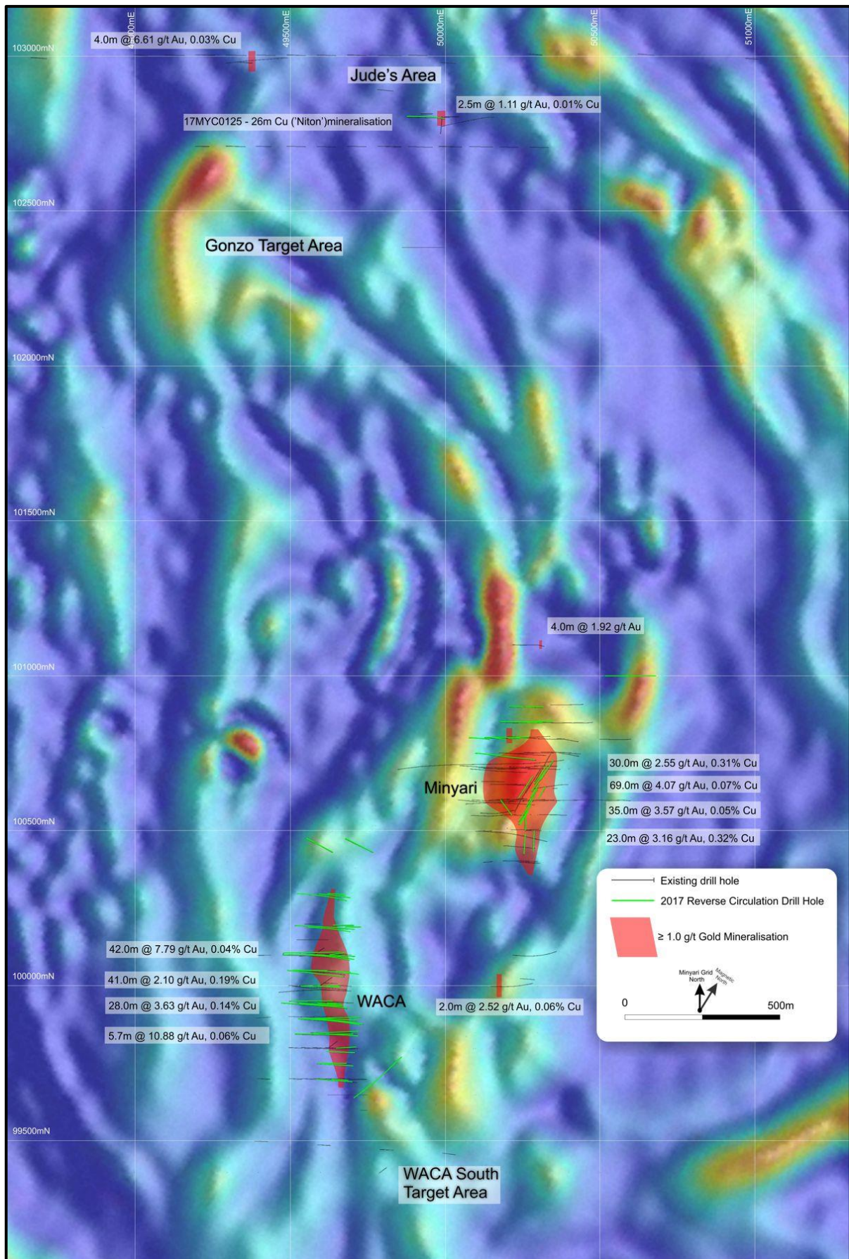
Figure 7: Minyari Dome plan view showing drillhole distribution, prospect and deposit locations.
