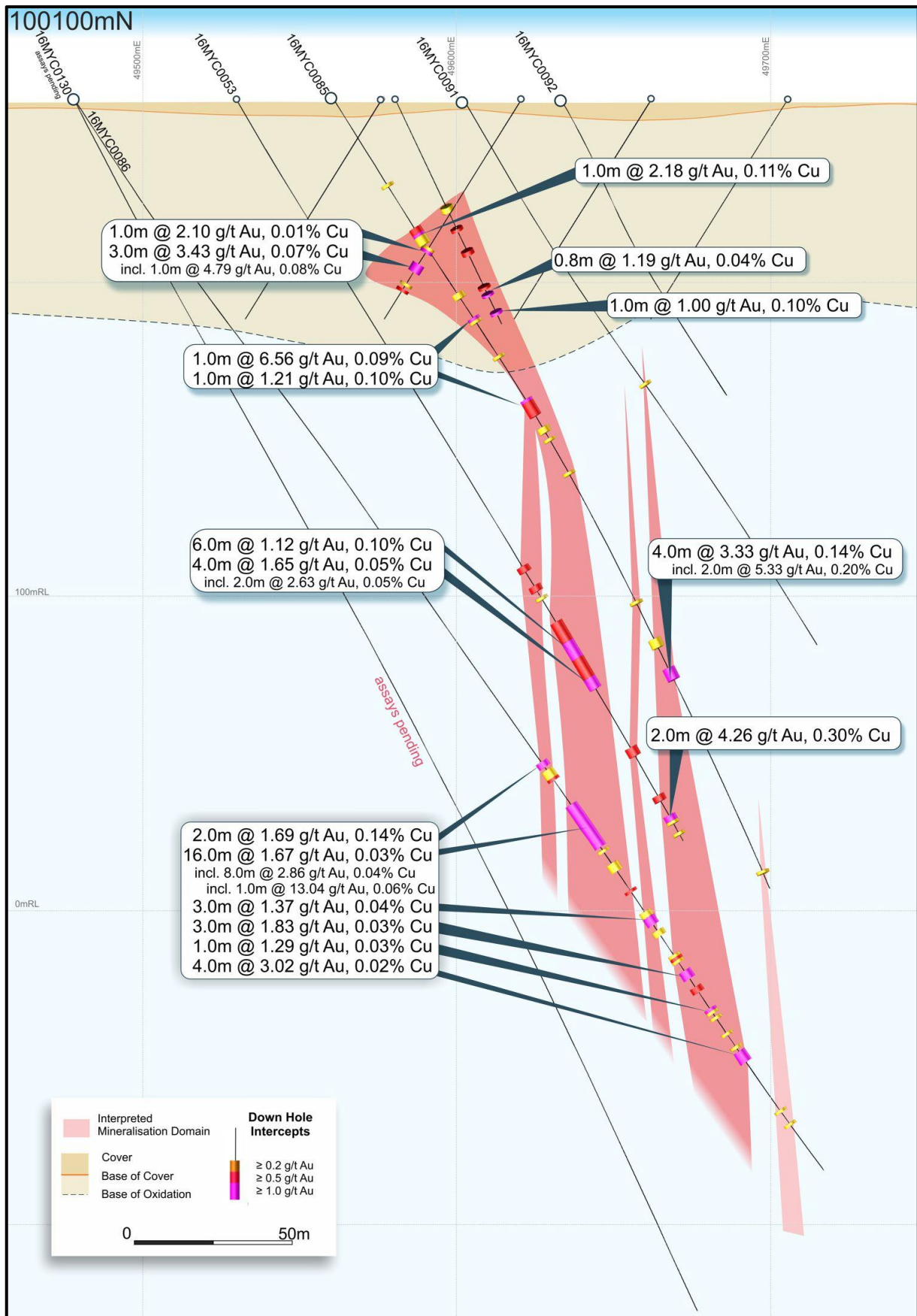
Figure 5: WACA Deposit 100,100 North interpreted (schematic) cross-section showing drill holes, including 2017 Phase 1 RC drill holes, with gold grade bars and interpreted gold-copper mineralisation domains (100m Local Grid – looking north).
