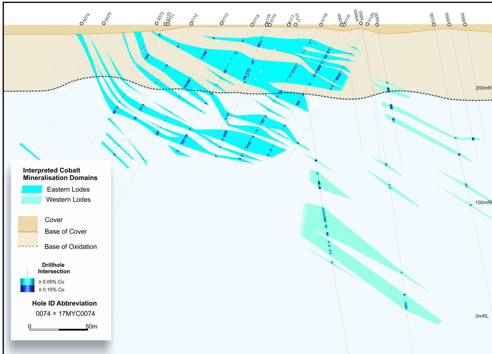
Figure 4: Minyari Deposit 'Longitudinal' Section showing only 2017 Phase 1 drill holes. Shows shallow north plunging eastern and western cobalt shoots (which are broadly coincident with the gold-copper mineralisation) along a +400m strike length of the Minyari deposit gold mineralisation zone (100mRL Local Grid – looking toward a bearing of 290° or WNW).
