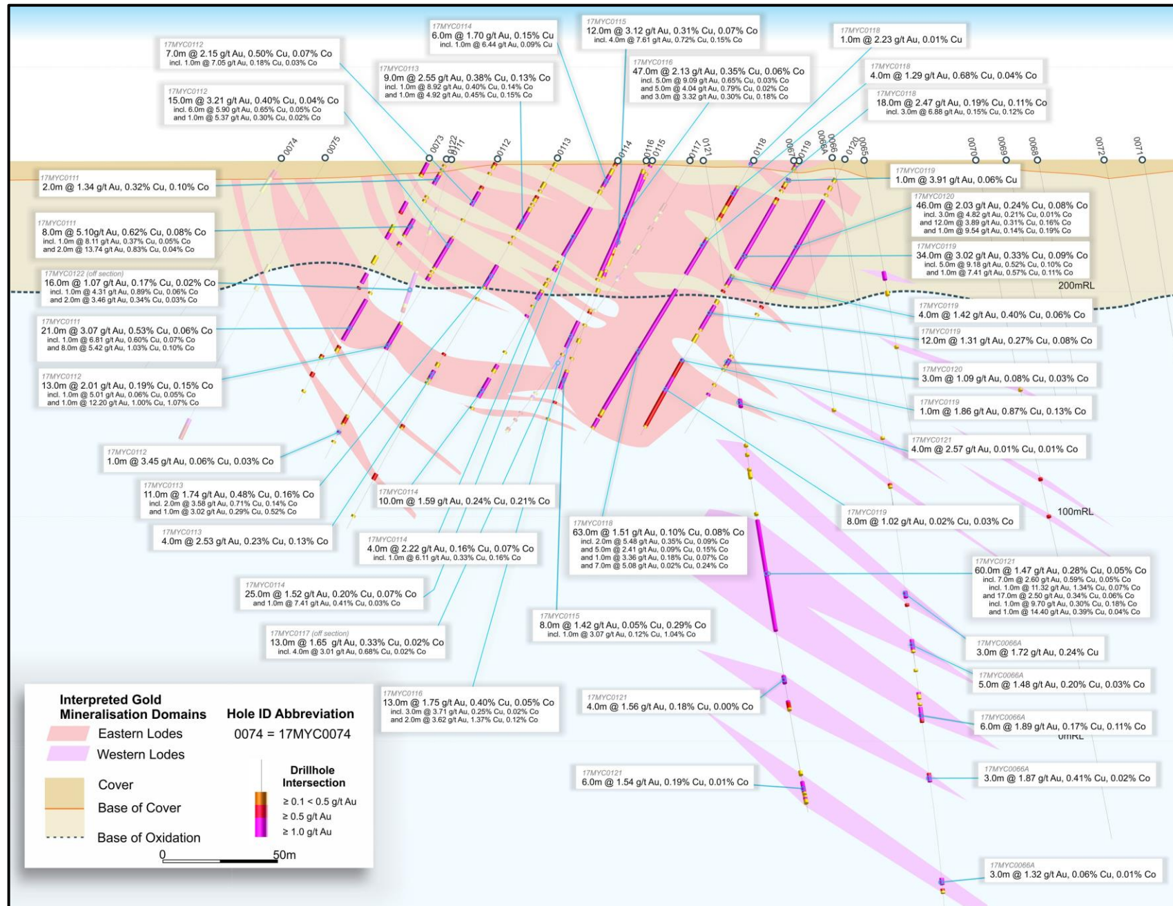
Figure 1: Minyari Deposit 'Longitudinal' Section showing only 2017 Phase 1 drill holes. Shows shallow north plunging high-grade eastern and western gold-copper-cobalt shoots along a +400m strike length of the Minyari deposit gold mineralisation zone (100mRL Local Grid – looking toward a bearing of 290° or WNW).
