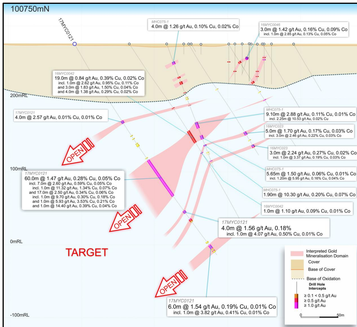
Figure 2: Minyari Deposit 100,750 North interpreted (schematic) cross-section showing drill holes, including 2017 Phase 1 RC drill holes, with gold grade bars and interpreted gold-copper-cobalt mineralisation domains (100m Local Grid – looking north).
