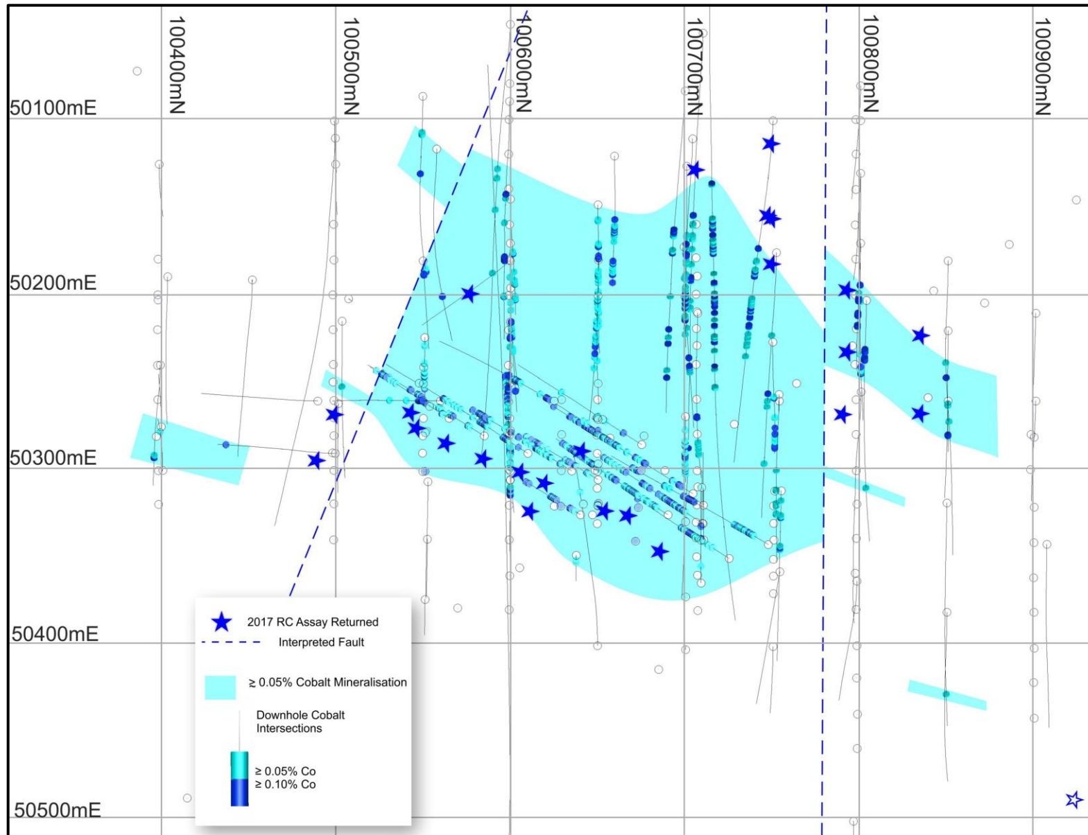
Figure 5: Minyari Deposit plan view showing drill hole locations and generalised plan projection of approximate boundary encapsulating \geq 0.05\% cobalt mineralisation (which is broadly coincident with the gold-copper mineralisation). (100m Local Grid).
