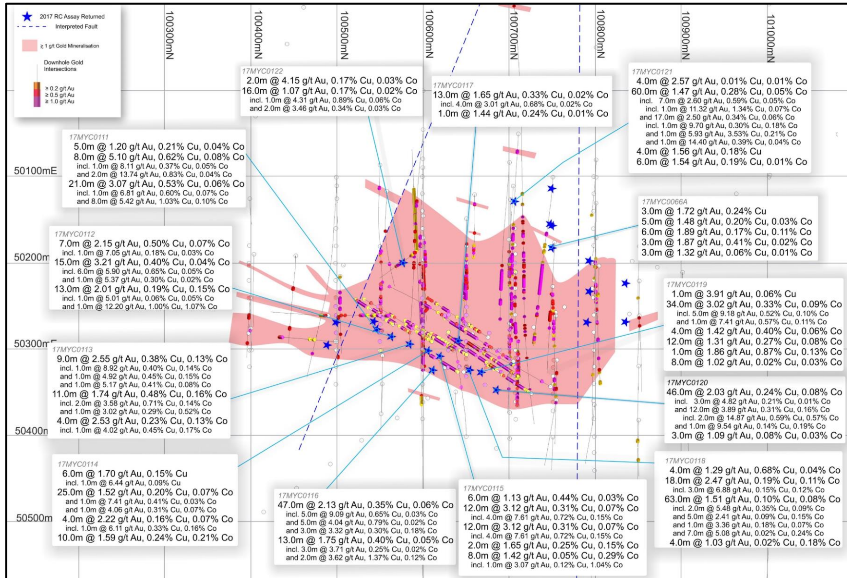
Figure 3: Minyari Deposit plan view showing drill hole locations and generalised plan projection of approximate boundary encapsulating 1.0 g/t gold mineralisation (which is broadly coincident with the copper-cobalt mineralisation). (100m Local Grid).
