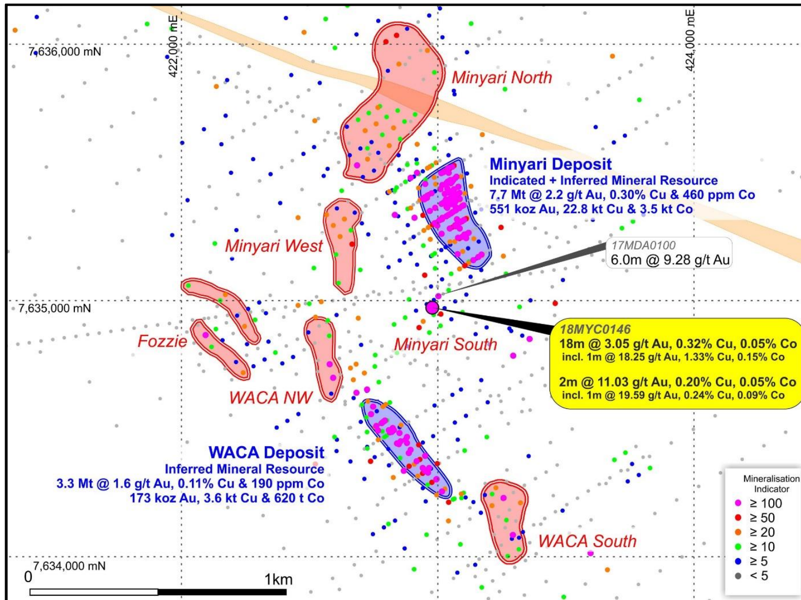
Figure 1: Plan view of the southern region of the Minyari Dome showing prospects, deposits and target locations, and drill holes annotated by “Mineralisation Indicator” (i.e. Au \text{ ppm} \times 100 + Ag \text{ ppm} \times 10 + Bi \text{ ppm} + Cu \text{ ppm}/100 + Co \text{ ppm}/100 + As \text{ ppm}/100 ) maximum value within 60m of surface. Regional GDA94 / MGA Zone 51 co-ordinates, 1km grid.
