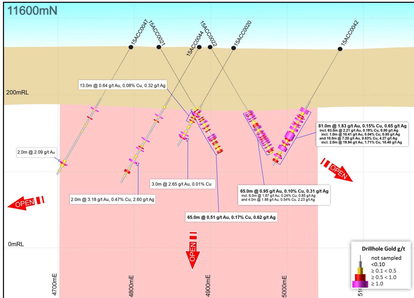
Figure 4: Calibre Deposit 11600 North interpreted (schematic) cross-section showing drill hole Au-Cu-Ag intersections. NB: 100m grid – North looking Calibre Local Grid.
