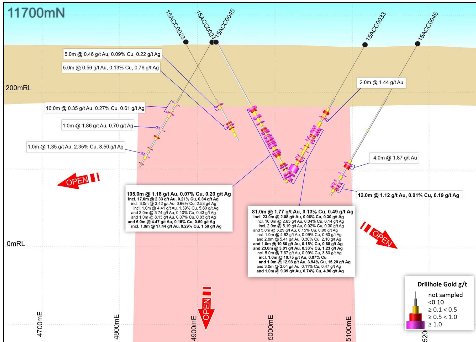
Figure 3: Calibre Deposit 11700 North interpreted (schematic) cross-section showing drill hole Au-Cu-Ag intersections. NB: 100m grid – North looking Calibre Local Grid.
