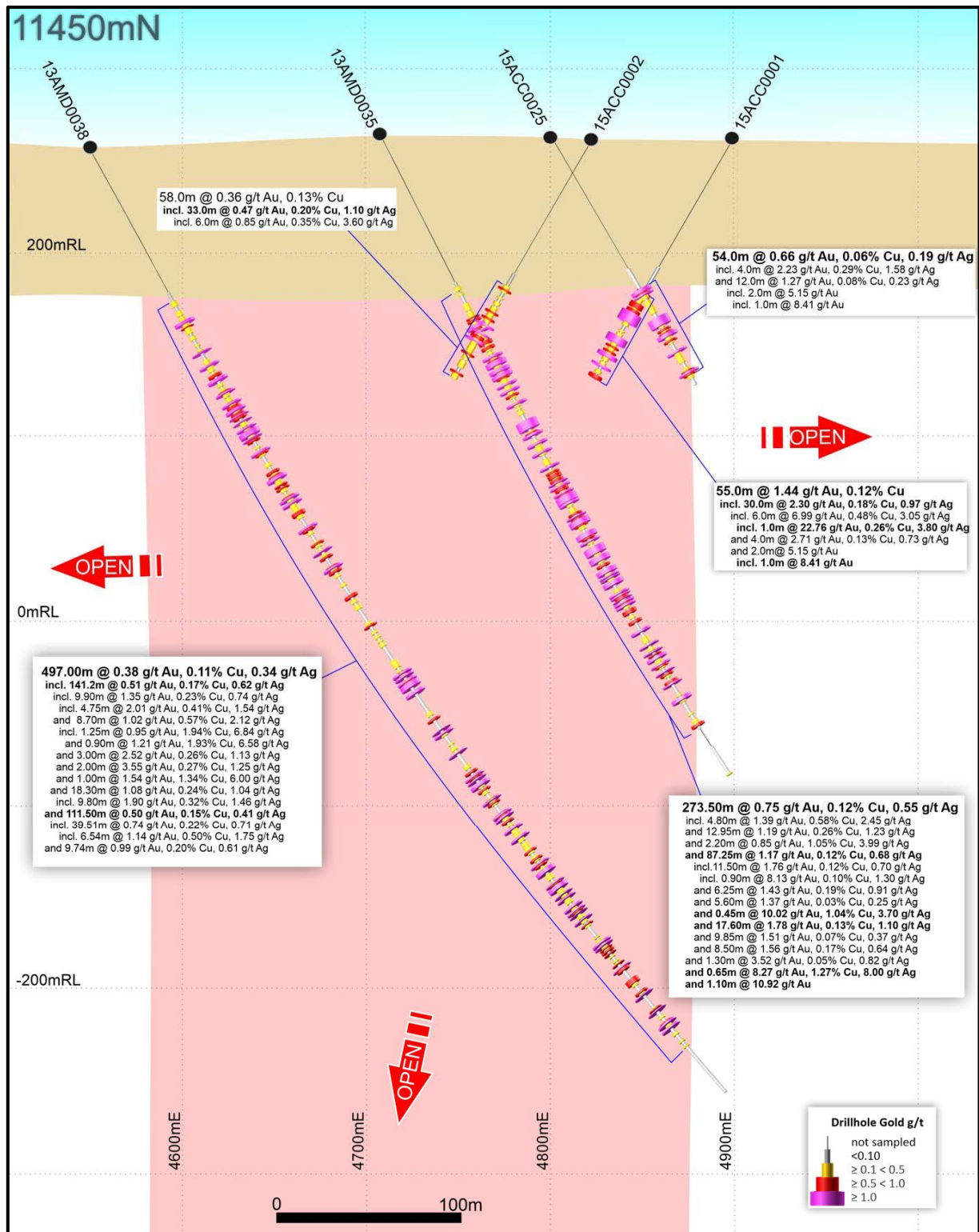
Figure 5: Calibre Deposit 11450 North interpreted (schematic) cross-section showing drill hole Au-Cu-Ag intersections. NB: 100m grid – North looking Calibre Local Grid.
