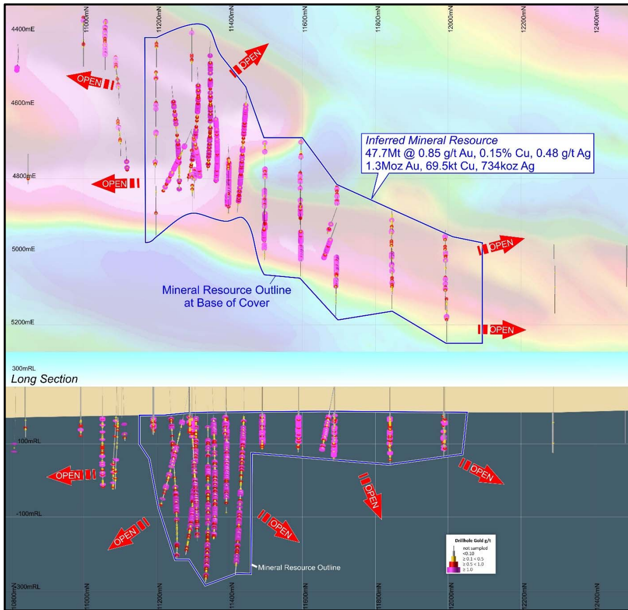
Figure 2: Calibre Deposit Plan over aeromagnetic image and west looking Vertical Projection showing all Calibre drill holes and depicting gold grade distribution. NB: 100m Calibre Local grid.
