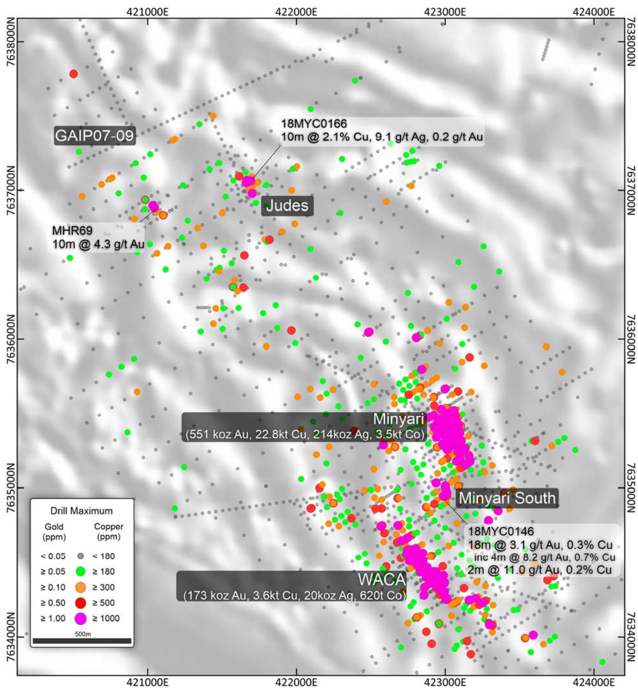
Figure 4: Map of the southern region of the Minyari Dome Project showing Minyari and WACA resource locations, Judea prospect and GAIP07-09 target locations, and drill hole maximum downhole gold and copper. NB: Over Airborne magnetic image (50m flight-line spacing at an altitude of 30m; grey-scale TMI-RP) and Regional GDA2020 / MGA Zone 51 co-ordinates, 1km grid.
