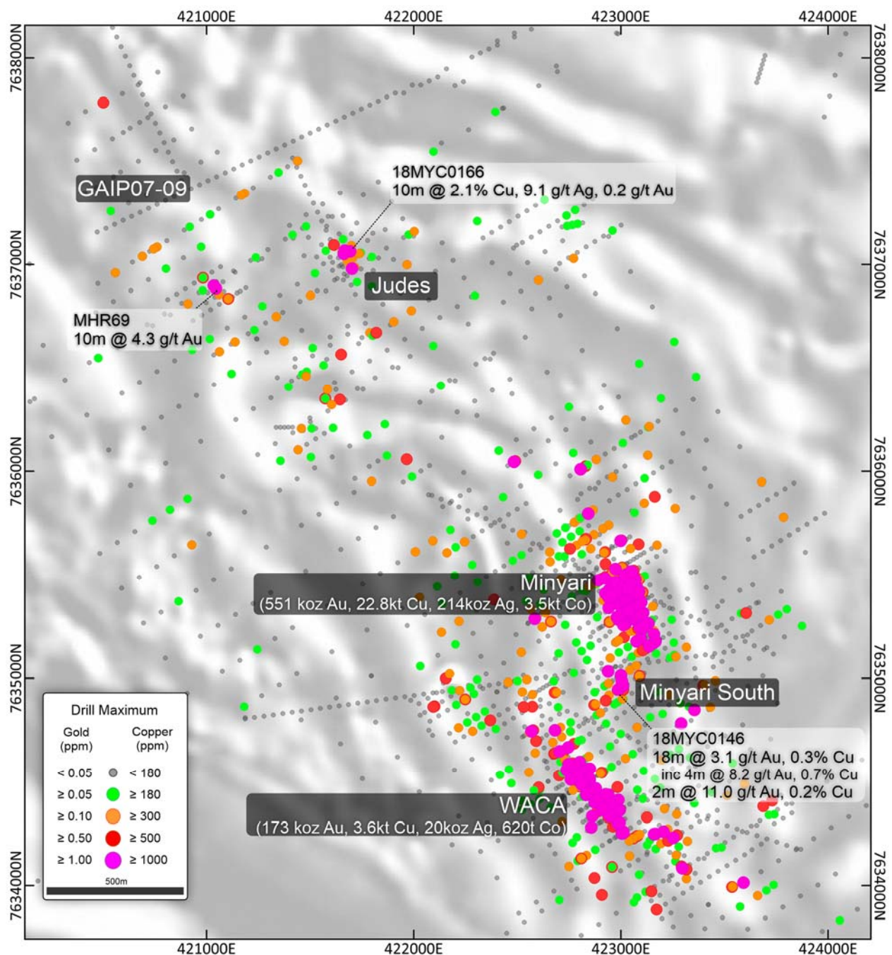
Figure 10: Map of the southern region of the Minyari Dome Project showing Minyari and WACA resource locations, Jude's project and GAIP07-09 target locations, and drill hole maximum downhole gold and copper. NB: Over Airborne magnetic image (50m flight-line spacing at an altitude of 30m; grey-scale TMI-RP) and Regional GDA2020 / MGA Zone 51 co-ordinates, 1km grid.
