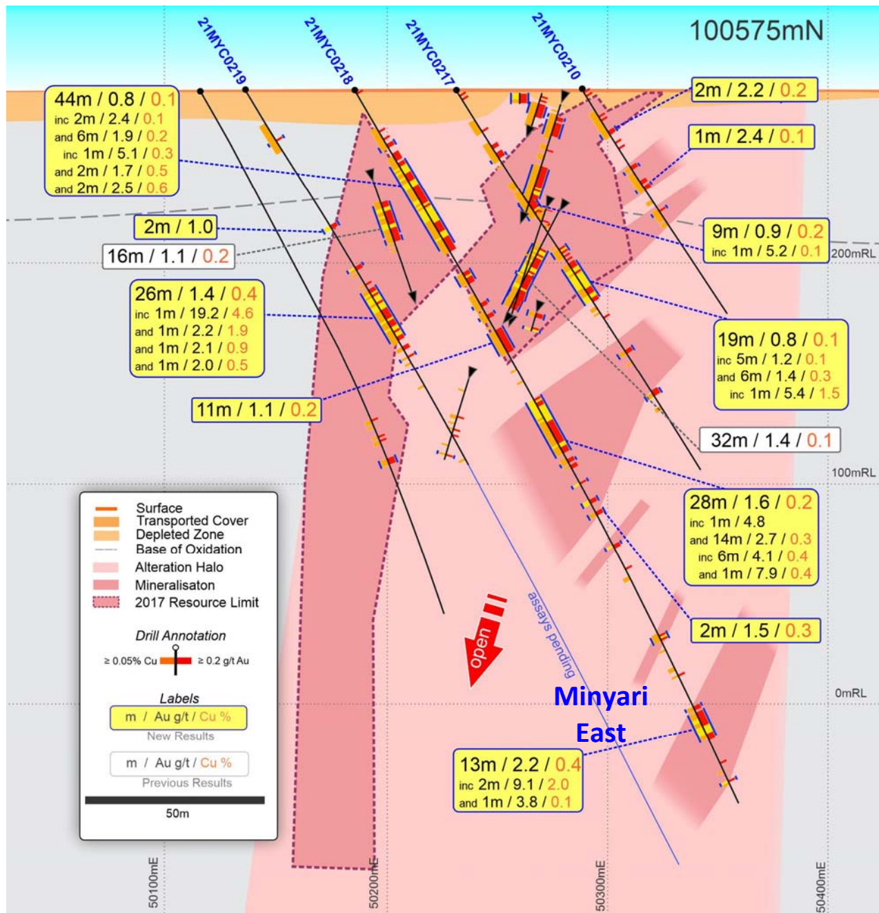
Figure 6: Minyari gold-copper-silver-cobalt deposit 100,575mN cross-section showing high-grade gold drill intercepts, with the deposit open down dip and along strike/plunge.
